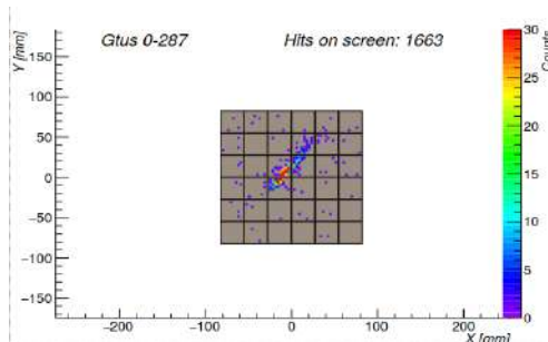
Simulated EAS
