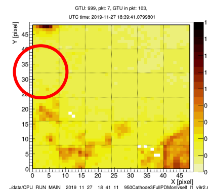
Meteors
